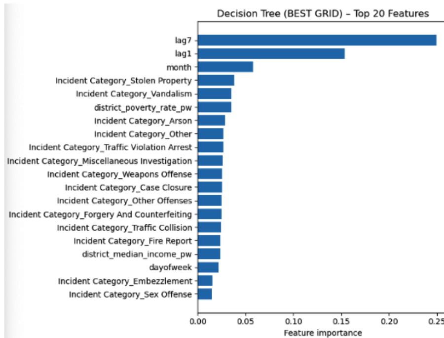
Figure 5. Top 20 feature importances for the tuned Decision Tree classifier (BEST GRID).
